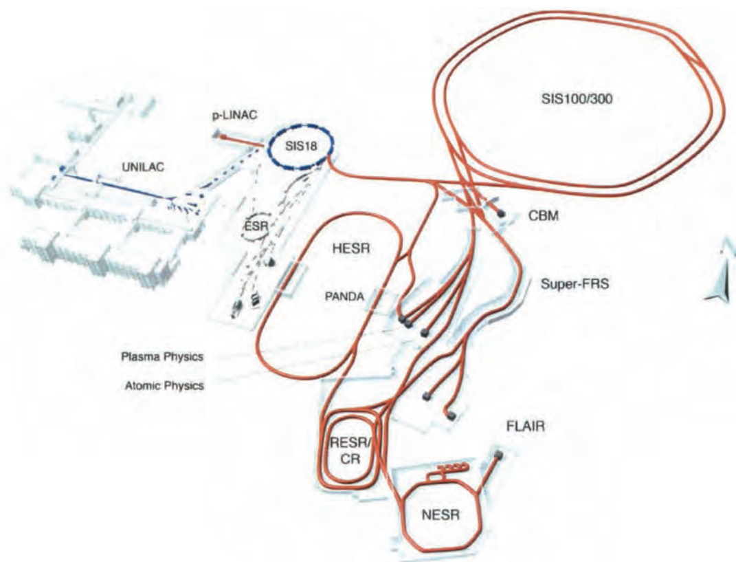
Figure 1: Layout of the FAIR facility: The existing accelerators at GSI (on the left in blue) act as injector for the new accelerator systems to be constructed (on the right in red).
