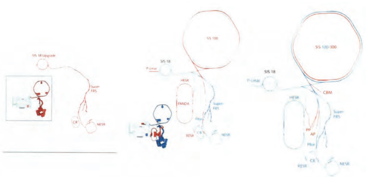
Figure 3: Stages of construction and operation of the FAIR facility. At stage 1 (left), only items marked in red will be constructed. The insert shows the civil construction taking place at stage 1. At stage 2 (middle), items drawn in red will be constructed whereas accelerator components in blue will already be operating. Buildings drawn in blue will exist already. At stage 3(right), no more civil construction will take place, and the accelerator components in red will be constructed.
